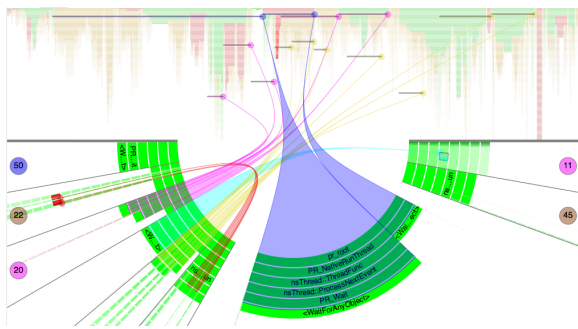
Figure 10: SyncTrace [KTD13] visualization shows thread call stacks and relationships between them. Image courtesy of B. Karran.
