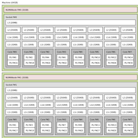
Figure 4: The output of lstopo , a tool provided by hwloc [BCOM*10] to visualize hardware topology. The memory hierarchy is shown as a hierarchical space-filling layout, with larger resources at the root and smaller caches and processors at the leaves.
